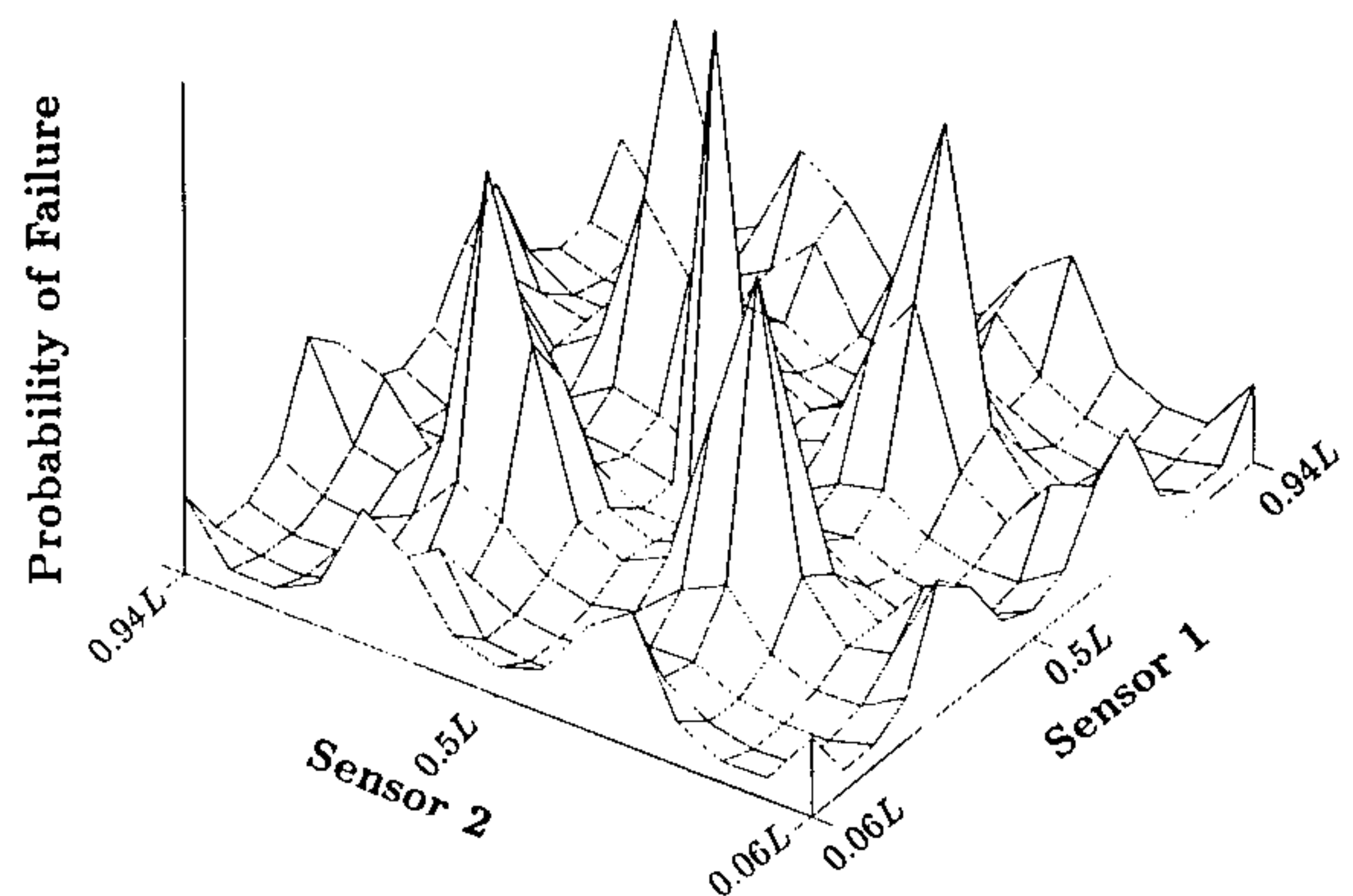
Figure 2. P_F against location of two sensors
